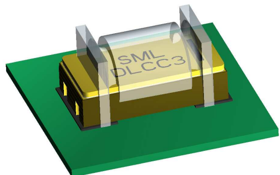
Image showing the DLCC3 on the recommended MELF-5.7 (D-5B) solder pad foot print and MELF-5.7 (D-5B) package overlay.
