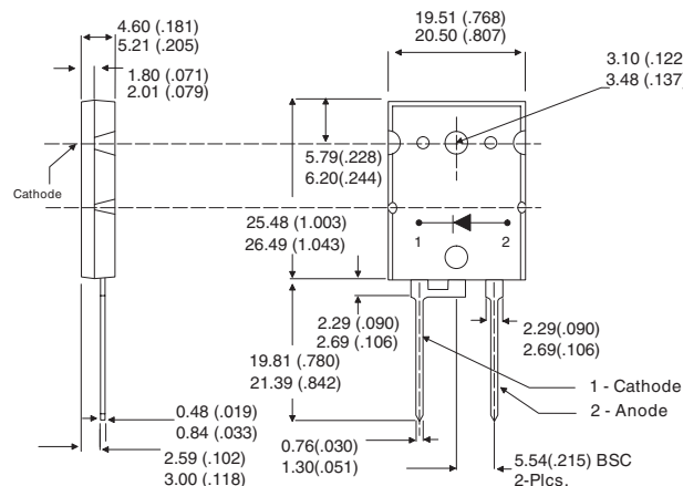
TO-264 Package Outline
