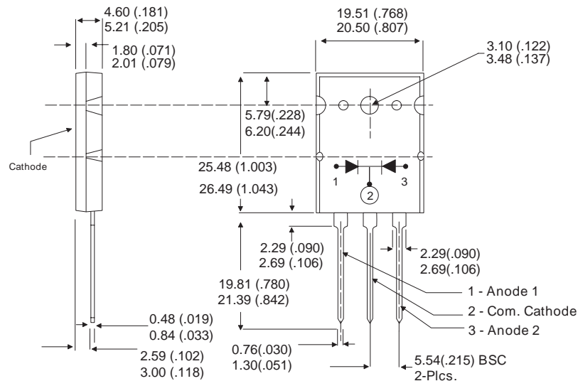
TO-264 Package Outline
